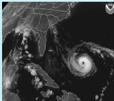
Hurricane Jeanne bears down on the State of Florida in September 2004.
